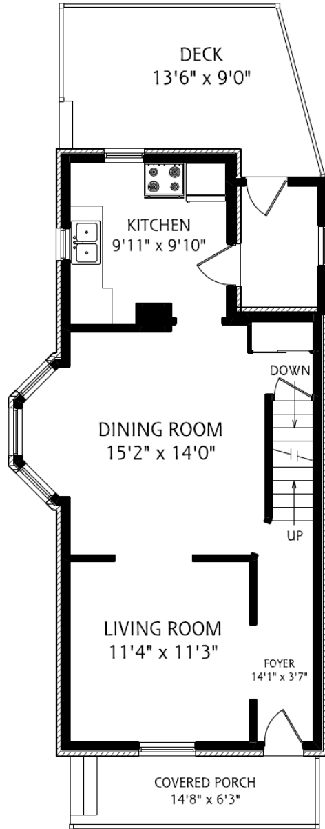
MAIN FLOOR 665 SQUARE FEET
